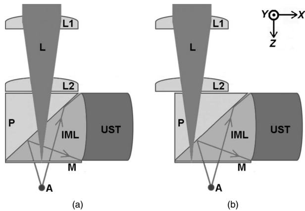
Fig. 1 Photoacoustic probe. L1: lens f=25 mm, optional L2: lens f=40 mm with radius of curvature=distance between L2 surface and optical focus, L: pulsed laser beam, P: 10 mm right-angle quartz silica prism, IML: index-matching liquid, UST: ultrasound transducer, M: fine membrane, A: Absorbing structure located in a turbid media. (a) Laser beam confocal with the ultrasound focus and (b) laser beam after translocation.
