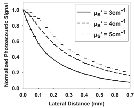
Fig. 2 Normalized photoacoustic signal as a function of lateral translocation distance for different \mu'_s . Error bars represent the standard deviation of 100 measurements.
